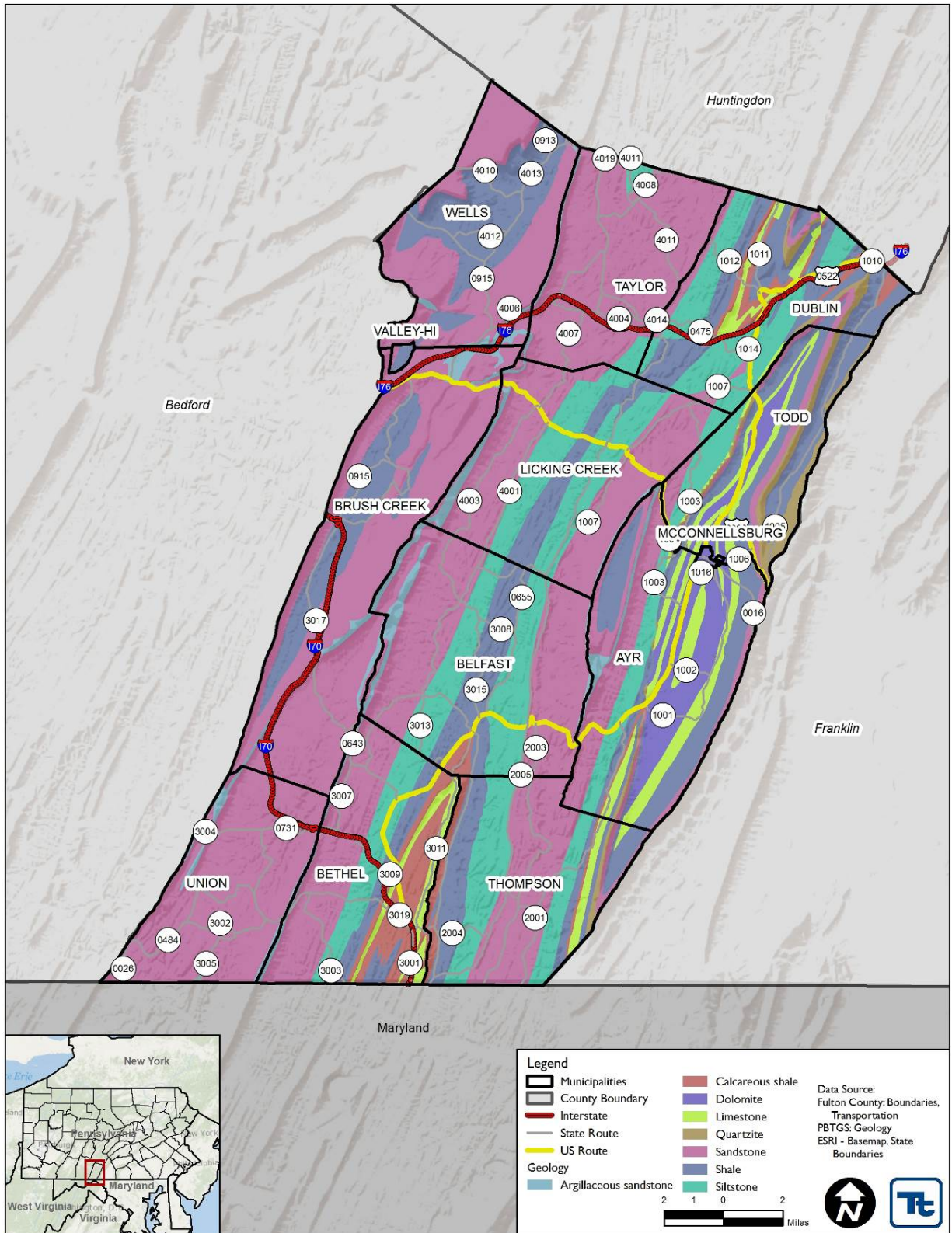
Figure 4.3.9-1. Fulton County Geology
